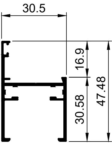
TCW3001 30.5 Frame 30.5mm Ix: 2.692cm 4
