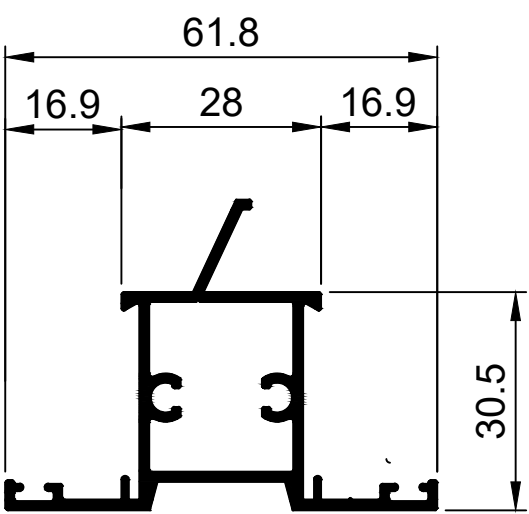
TCW3008 30.5 Mullion 30.5mm W/Bar Ix: 4.435cm 4
