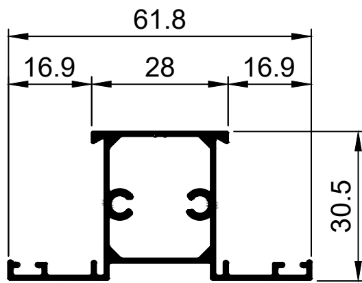
TCW3007 30.5 Mullion 30.5mm Lite Ix: 2.636cm 4
