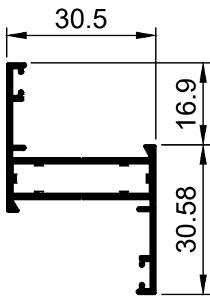
TCW3010 30.5 Sash Ix: 2.575cm 4
