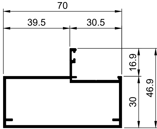
TCW3004 30.5 Frame 70mm Flat Back Ix: 19.530cm 4
