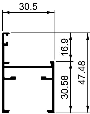
TCW3002 30.5 Frame 30.5mm Lite Ix: 2.243cm 4
