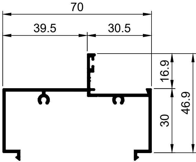
TCW3003 30.5 Frame 70mm Ix: 16.398cm 4
