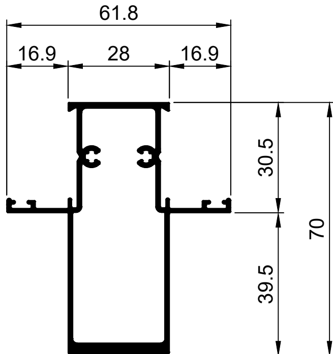
TCW3021 30.5 Mullion 70mm Ix: 24.033cm 4
