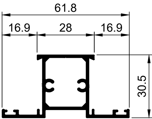
TCW3005 30.5 Mullion 30.5mm Ix: 3.223cm 4
