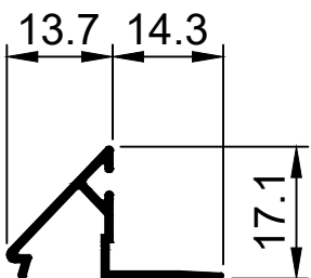
TCW3014 30.5 Bead Angled 6mm Glass Ix: 0.237cm 4
