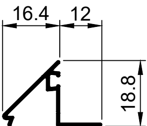
TCW3013 30.5 Bead Angled 4mm Glass Ix: 0.274cm 4
