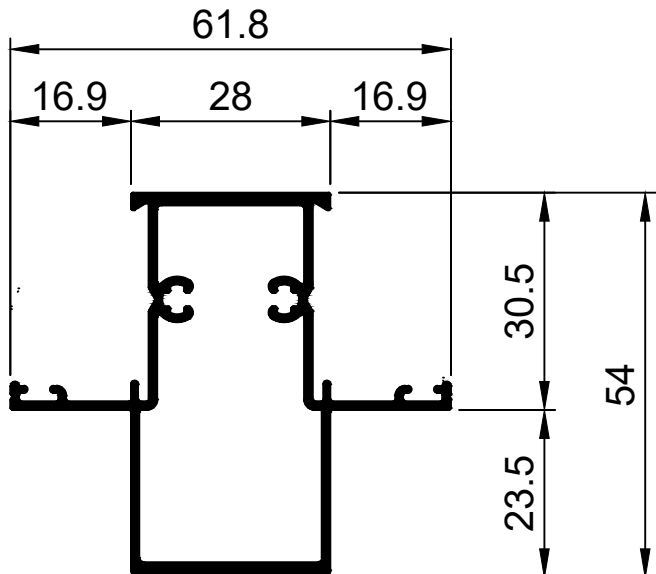
TCW3020 30.5 Mullion 54mm Ix: 10.505cm 4
