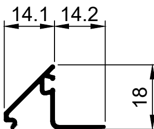
TCW3015 30.5 Bead Angled Multi 13mm Gap Ix: 0.278cm 4
